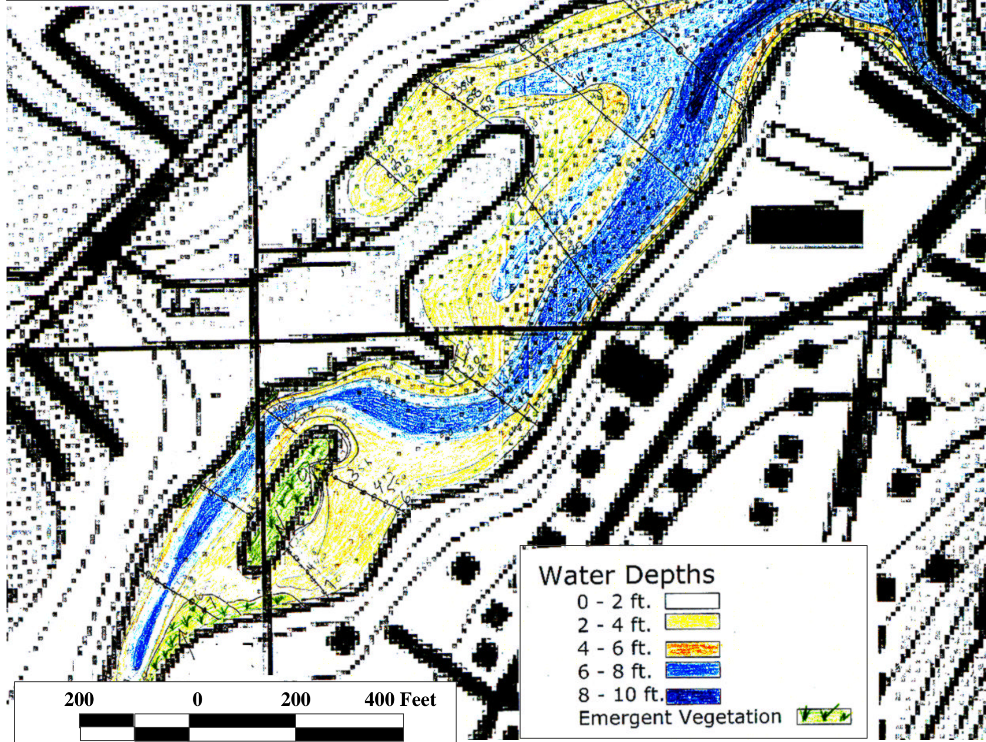
Figure 6-2 Assabet River: Bathymetry of Rt 85/Hudson Impoundment, Hudson (RM 18.5)
